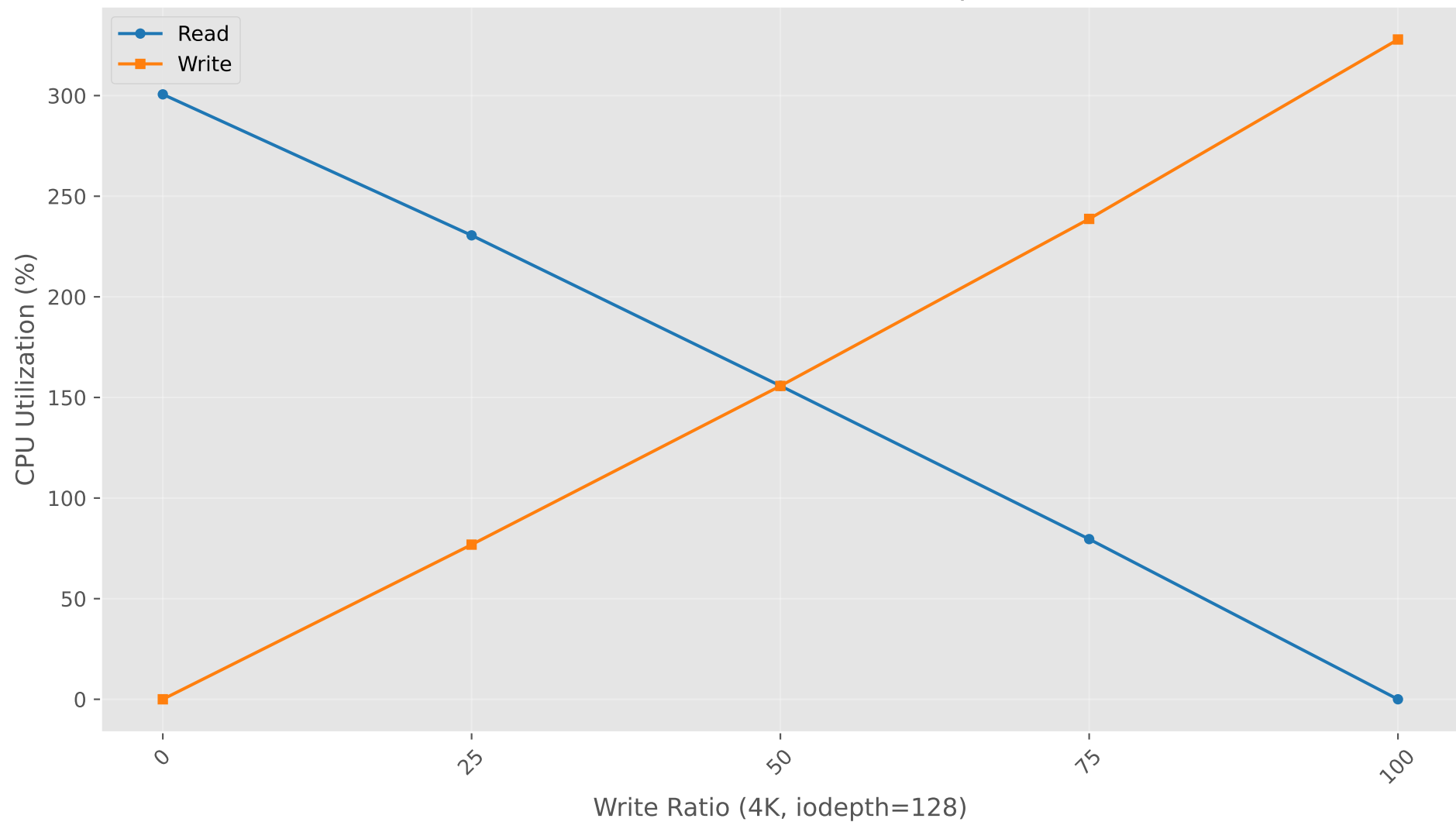
CPU Total vs Write Ratio (4K, iodepth=128)
